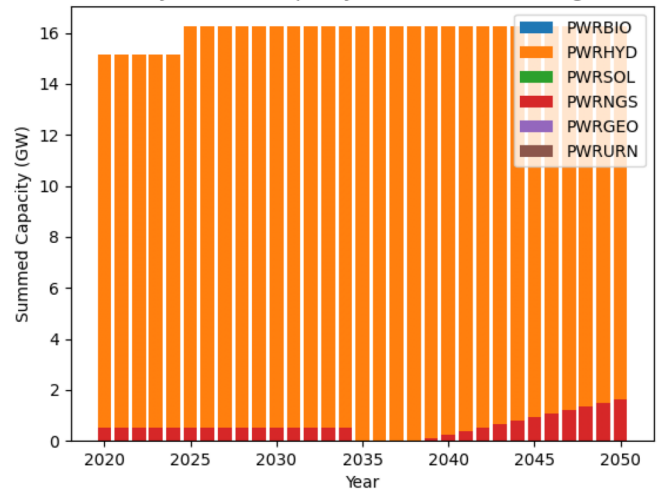
Yearly Summed Capacity for Different Technologies
