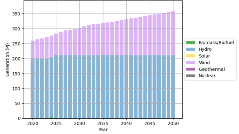
Yearly Generation for Different Technologies - REF Case
